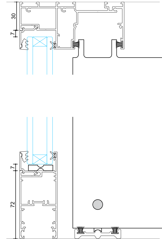
Section B Vertical Section Scale: 1:2
