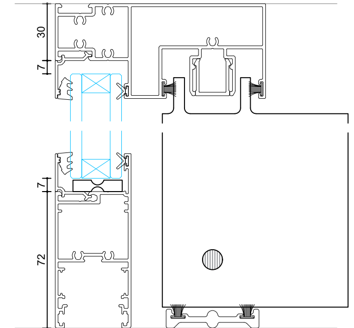
Section C Vertical Section Scale: 1:2
