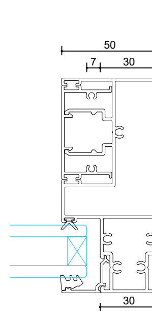
Section A Horizontal Section Scale: 1:2
