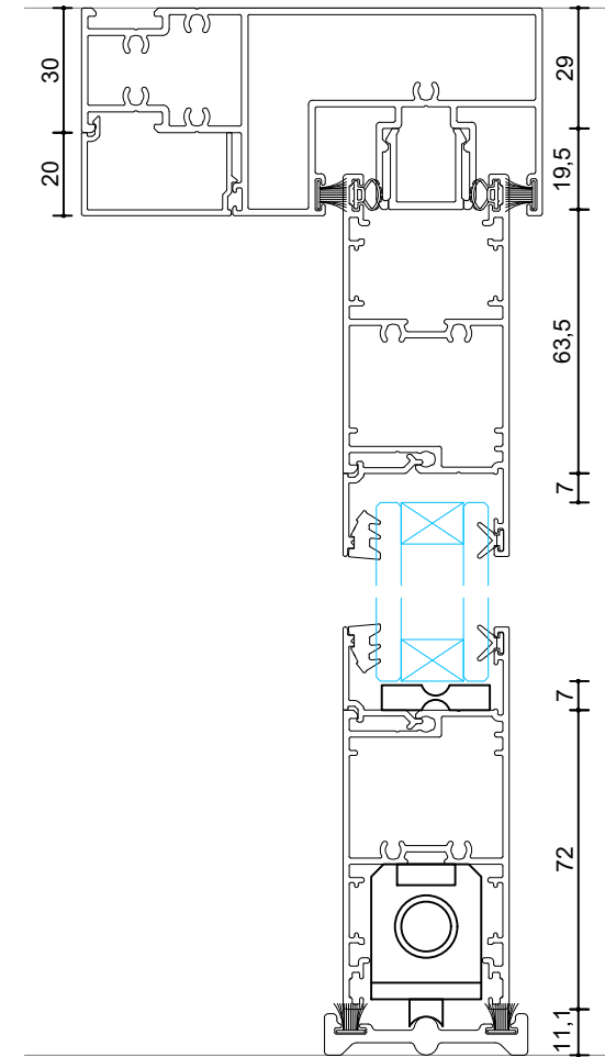
Section B Vertical Section Scale: 1:2
